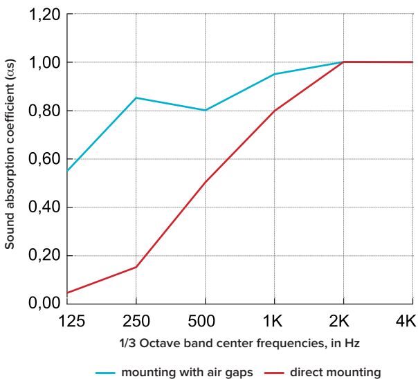
ATMOtex 25 mm
