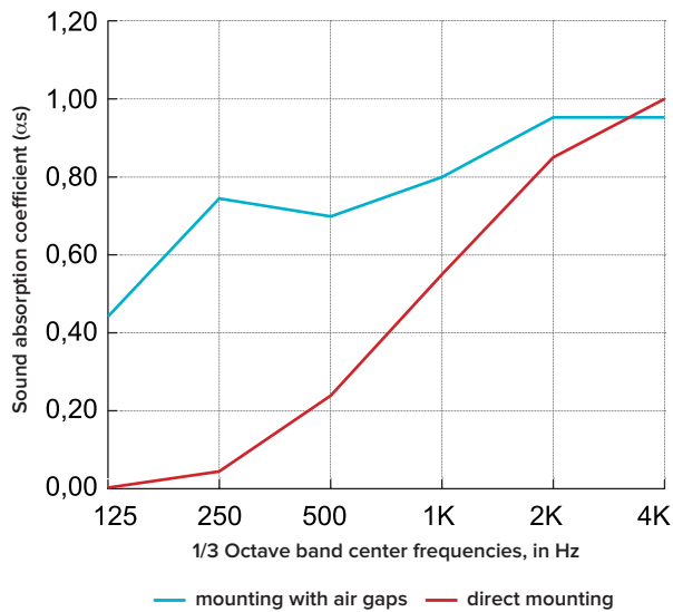
ATMOtex 10 mm
