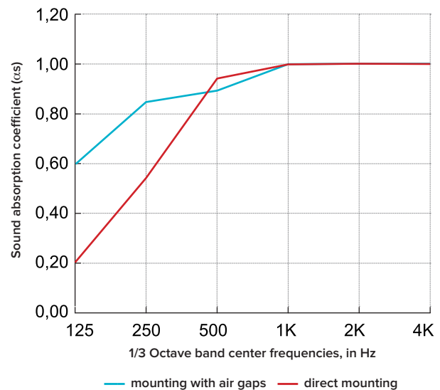
ATMOtex 40 mm
