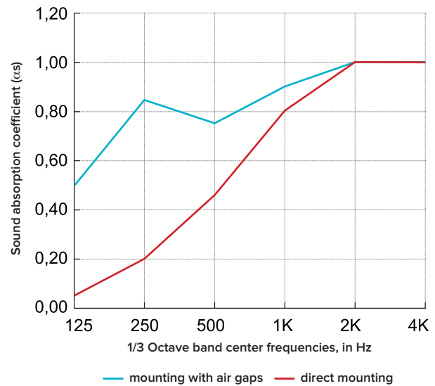
ATMOtex 20 mm
